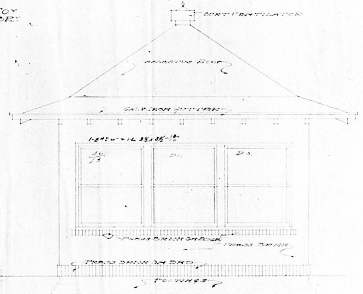
SIDE ELEVATION
