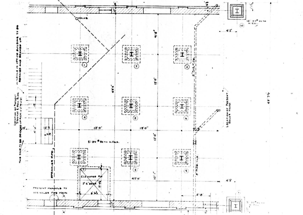
1 ST FLOOR & PIER PLAN.
