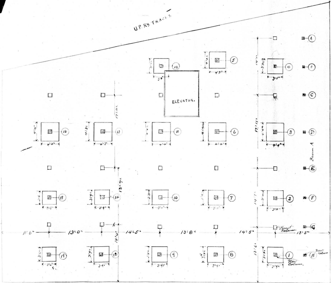
BASEMENT PLAN. OMAHA BASKET STORES & WARE HOUSE BETTERMENTS. SCALE 7/8" JOHN H. HANDE CONTRACTOR OMAHA NEB.
